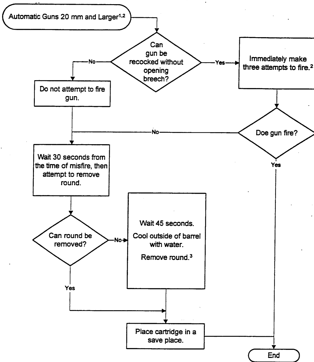
Figure C14.F2. Misfire of Automatic Guns, 20 mm and Larger.
